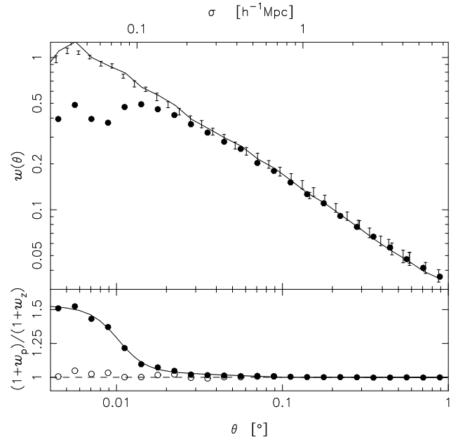
Figure 2. Top panel: w(\theta) for the mean of the NGP and SGP redshift catalogues (solid points), the mean of the masked parent catalogues (solid line), and the full APM result (error bars). Bottom panel: The parent catalogue result divided by the redshift catalogue results (uncorrected - solid points; collision corrected (see Section 3.3) - open points). The solid line is the curve used to correct the fibre collisions. The top axis converts \theta into a projected separation, \sigma , at the effective redshift of the survey, z_s = 0.15 .
