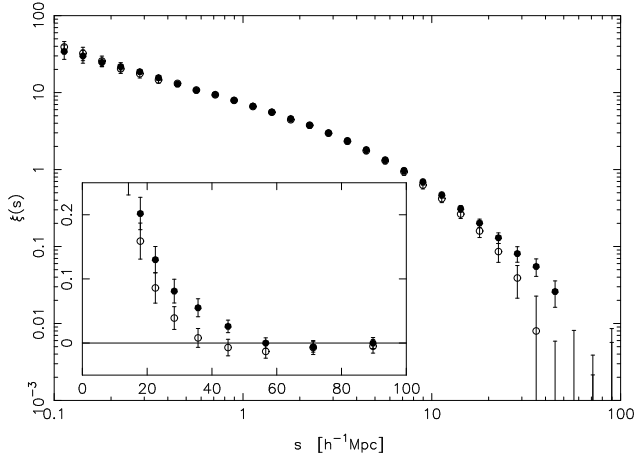
Figure 5. The redshift-space correlation function for the NGP (open points) and SGP (solid points) 2dFGRS data with error bars from the rms of mock catalogue results. Inset plotted on a linear scale.
