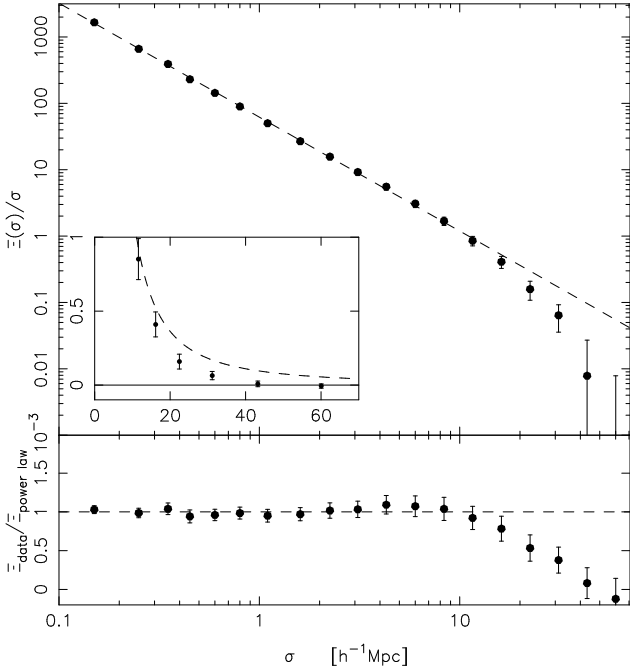
Figure 9. Top panel: The projected correlation function of the combined data with error bars from the rms spread between mock catalogue results. The dashed line is the best-fit power-law for 0.1 < \sigma < 12 h^{-1}\text{Mpc} ( r_0 = 4.98 , \gamma_r = 1.72 , A = 3.97 ). Inset is plotted on a linear scale. Bottom panel: The combined data divided by the power-law fit.
