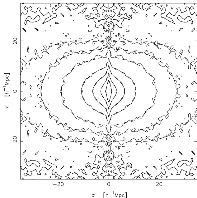
Figure 22. Contours of \xi(\sigma, \pi) for the 2dFGRS combined data (solid lines) and the best-fit model (see Table 3) using the Hubble Volume \xi(r) fitted to scales 8 < s < 30 h^{-1}\text{Mpc} (dashed lines). Contour levels are at \xi = 4.0, 2.0, 1.0, 0.5, 0.2, 0.1, 0.05 and 0.0 (thick line).
