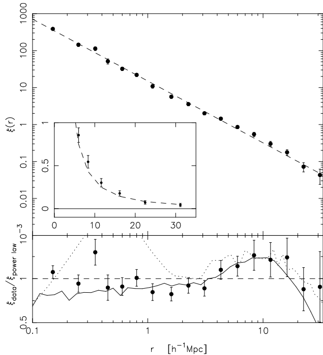
Figure 11. Top panel: The real-space correlation function of the combined 2dFGRS using the method of S92, with error bars from the rms spread between mock catalogues. The dashed line is the best-fit power law ( r_0 = 5.05 , \gamma_r = 1.67 ). Inset is plotted on a linear scale. Bottom panel: The data divided by the power law fit. The solid line is the de-projected APM result (Padilla & Baugh 2003) as discussed in the text. The dotted line is the result from the Hubble Volume.
