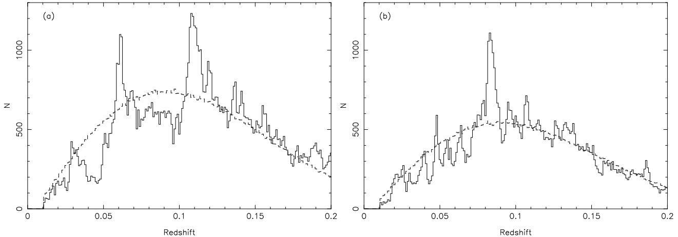
Figure 3. Redshift distributions, N(z) , for the 2dFGRS data (solid lines) and the normalised random catalogues generated using the survey luminosity function (dashed lines) for the (a) SGP and (b) NGP.
