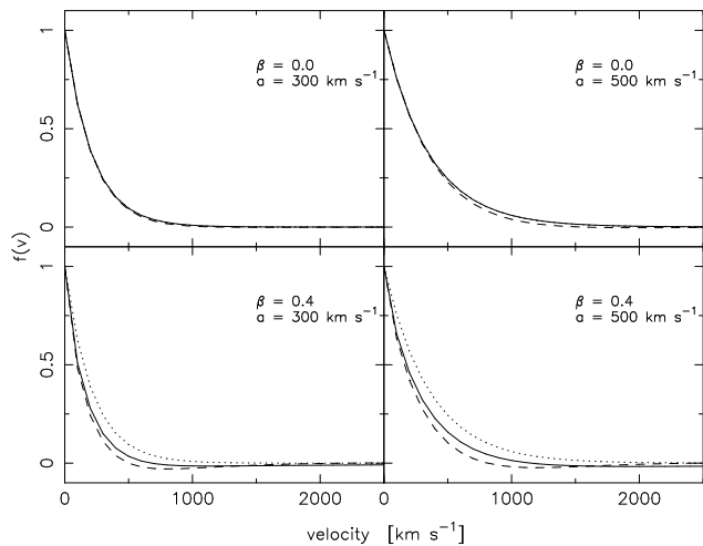
Figure 17. The peculiar velocity distribution for various models (see labels). The solid line is the recovered distribution for a model with no smoothing and using all scales < 70 h^{-1}\text{Mpc} . The dashed line is the recovered distribution for a model cut at 32 h^{-1}\text{Mpc} and smoothed with a Hann window. The dotted line is the input exponential peculiar velocity distribution (this coincides with the solid line in the top panels).
