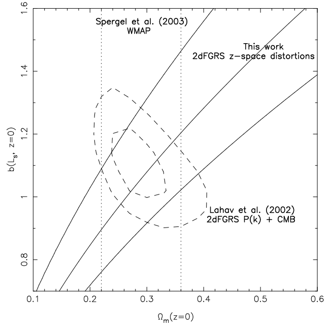
Figure 24. Constraints on \Omega_m and b - Solid lines: Best-fit and 1\sigma error contours on \beta from this work, evolved to the present day (see Section 8.1). Dashed lines: 1\sigma and 2\sigma error contours from Lahav et al. (2002). Dotted lines: 1\sigma constraints from WMAP (Spergel et al. 2003).
