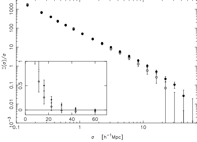
Figure 8. The projected correlation functions for the NGP (open points) and SGP (solid points) 2dFGRS data with error bars from the rms spread between mock catalogue results. Inset plotted on a linear scale.
