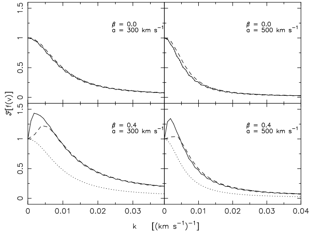
Figure 16. The Fourier transform of the peculiar velocity distribution for various parameters (see labels). The solid line is for a model with no smoothing and using all scales < 70 h^{-1}\text{Mpc} . The dashed line is for a model cut at 32 h^{-1}\text{Mpc} and smoothed with a Hann window (like L02). The dotted line is the Lorentzian equivalent of the input exponential peculiar velocity distribution (this coincides with the solid line in the top panels).
