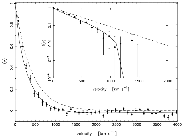
Figure 21. The combined 2dFGRS peculiar velocity distribution (solid points), compared to a pure exponential distribution with a = 570 \text{ km s}^{-1} (dashed line) and a model with a = 570 \text{ km s}^{-1} and \beta = 0.49 (solid line). The error bars are from the scatter in mock results.
