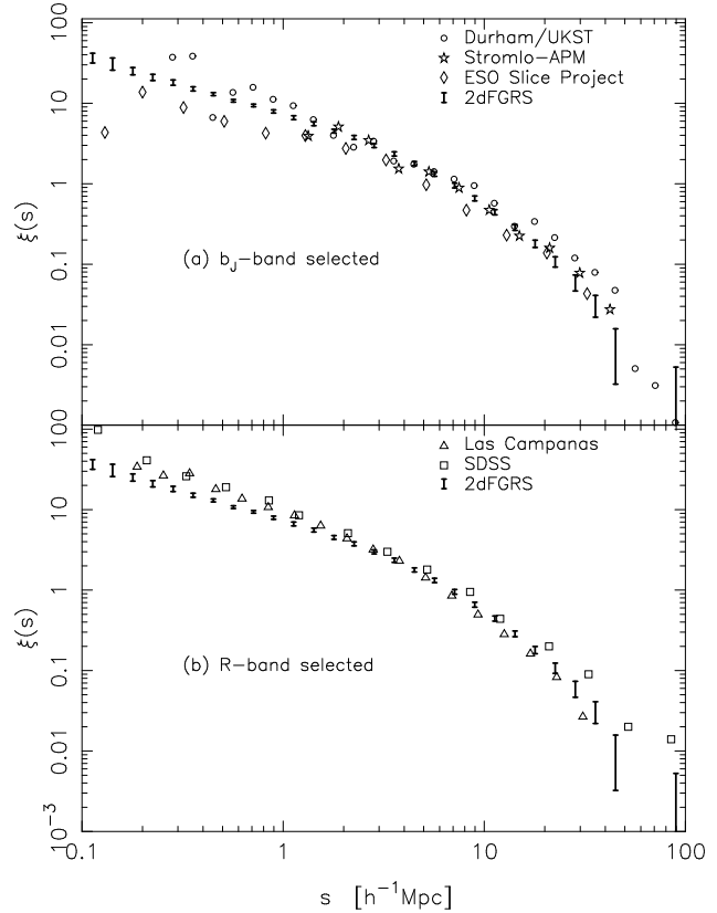
Figure 7. Comparison of 2dFGRS \xi(s) with (a) other b_J band selected surveys as indicated and (b) R band selected surveys as indicated. These results are discussed in the text.
