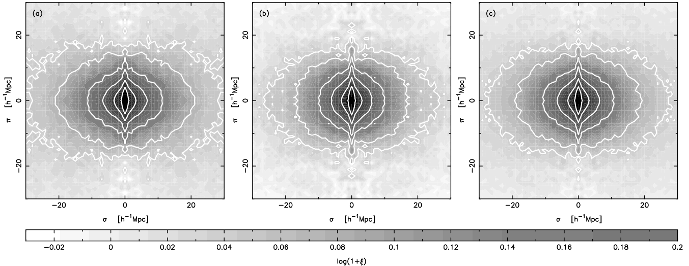
Figure 4. Grey-scale plots of the 2dFGRS \xi(\sigma, \pi) (in 1 h^{-1}\text{Mpc} bins) for (a) the SGP region, (b) the NGP region and (c) the combined data. Contours are overlaid at \xi = 4.0, 2.0, 1.0, 0.5, 0.2 and 0.1 .
