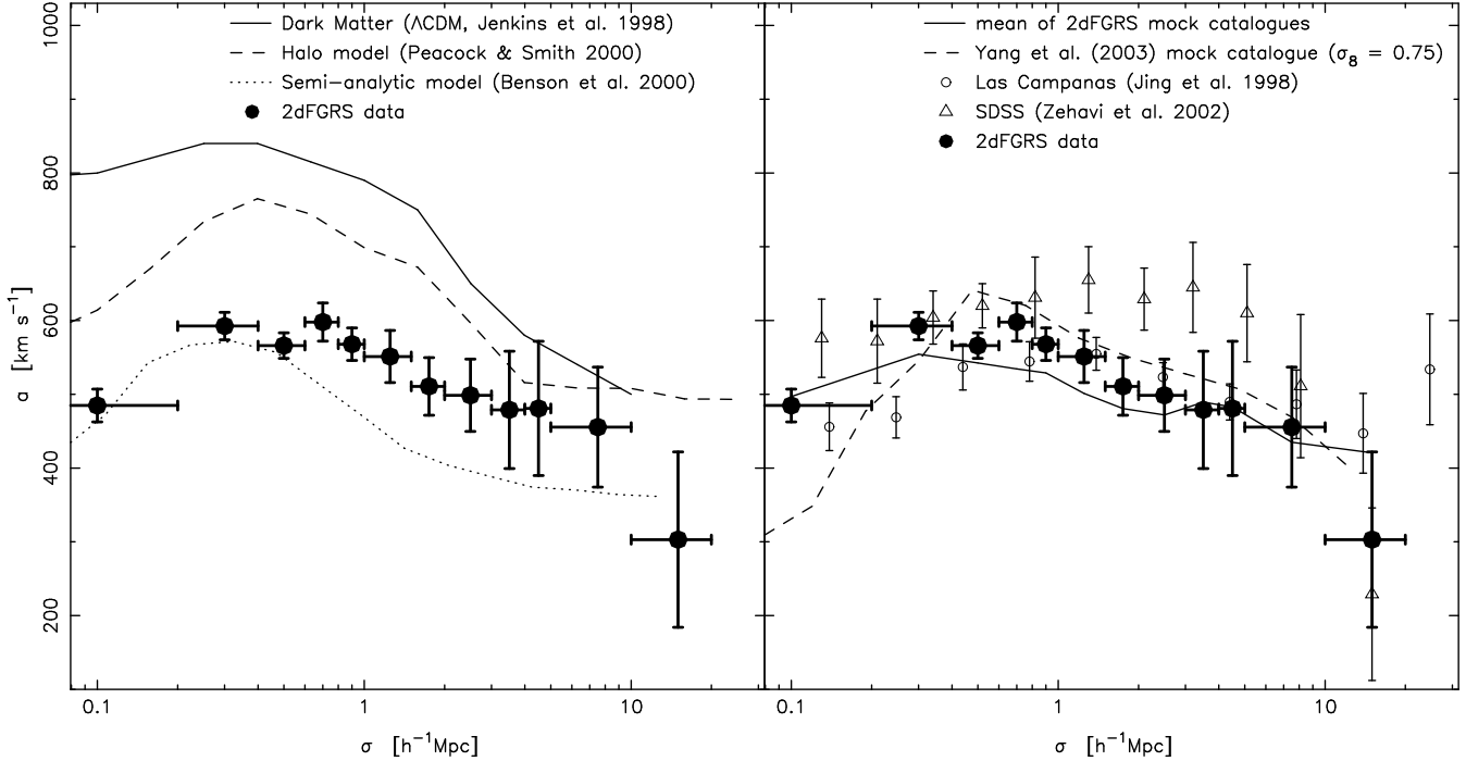
Figure 23. The variation of a with projected separation, \sigma . Left panel: 2dFGRS data compared to some analytical models, as indicated in the legend. Right panel: 2dFGRS data compared to other redshift surveys and simulated catalogues, as indicated in the legend. The 2dFGRS data and simulated catalogue results use \beta to calculate the infall velocities whereas the other results assume a functional form (see discussion in Section 7.4).
