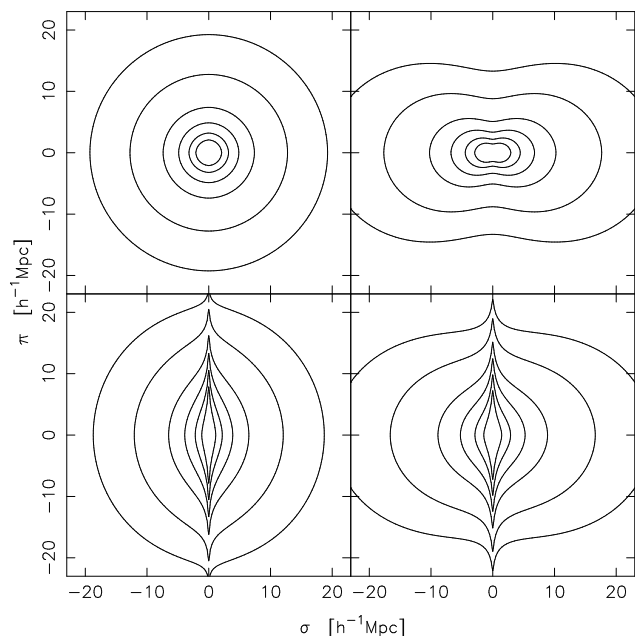
Figure 12. Plot of model \xi(\sigma, \pi) 's calculated as described in Section 4. The lines represent contours of constant \xi(\sigma, \pi) = 4.0, 2.0, 1.0, 0.5, 0.2 and 0.1 for different models. The top left panel represents an undistorted correlation function ( a = 0, \beta = 0 ), the top right panel is a model with coherent infall added ( a = 0, \beta = 0.4 ), the bottom left panel is a model with just random pairwise velocities added ( a = 500 \text{ km s}^{-1}, \beta = 0 ) and the bottom right panel has both infall and random motions added ( a = 500 \text{ km s}^{-1}, \beta = 0.4 ). These four models have r_0 = 5.0 h^{-1} \text{ Mpc} and \gamma_r = 1.7 .
