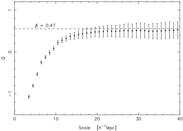
Figure 15. The mean Q factor for the mock catalogues with error bars from the rms spread in mock catalogue results. The dashed line is the true value of \beta = 0.47 . The slight bias is caused by the random peculiar velocities as discussed in the text.
